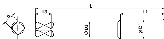
Reduced Shank (7/16" - 2")
